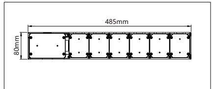
Tile Hole Dimensions
